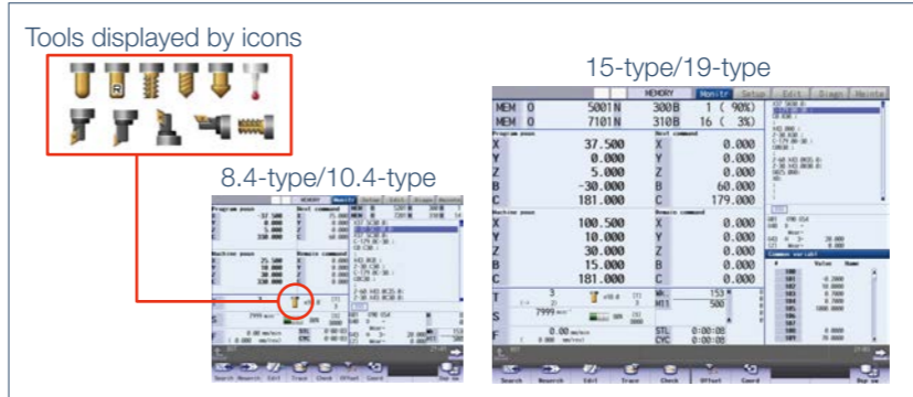
Various features and operation menus are indicated using easy-to-recognize icons. Tool icons tell you the tool type, left- or right-hand, lifetime and other information at a glance.
