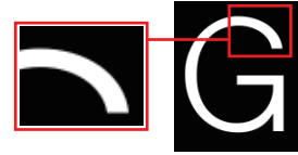
Antialiasing enabled
