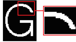
Antialiasing disabled
