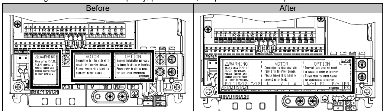
Note) Appearance of the product with the lower front cover removed
