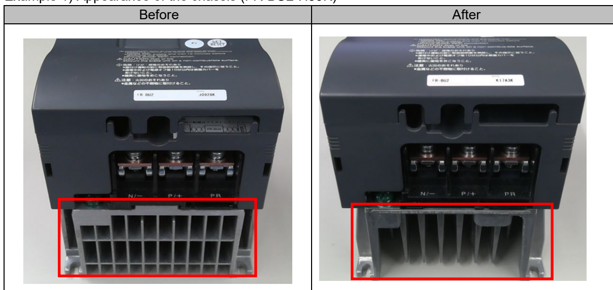
Example 1) Appearance of the chassis (FR-BU2-H30K)
