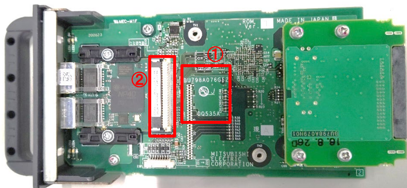
Board whole
