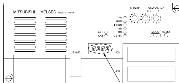
17-segment LED
