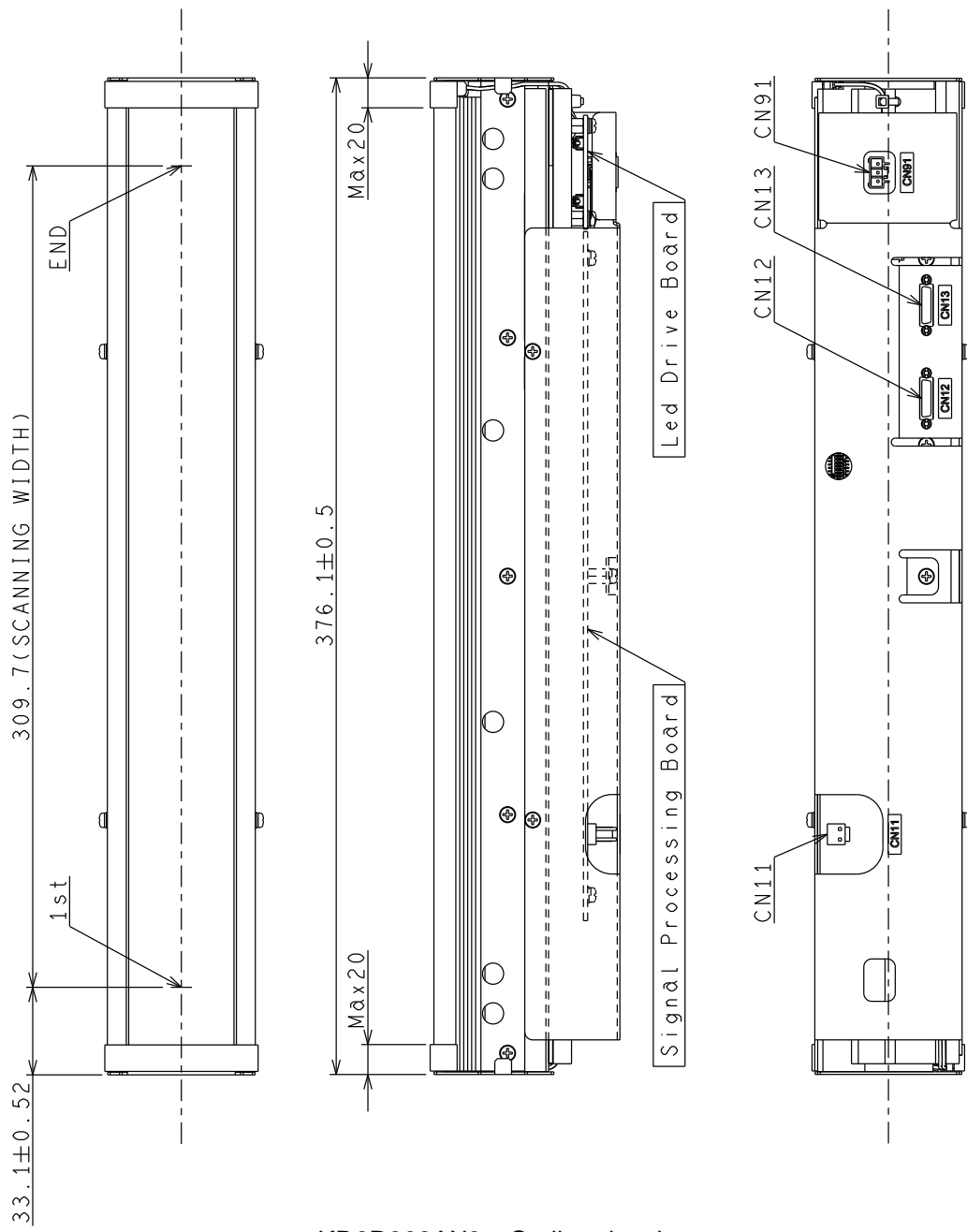
KD6R309AX3 Outline drawing
