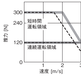
LM-H3P3D-48P-CSS0 (注1, 2, 3)
