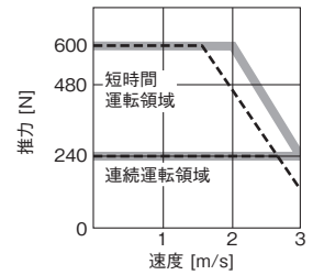
LM-H3P7D-96P-ASS0 (注1, 3)
