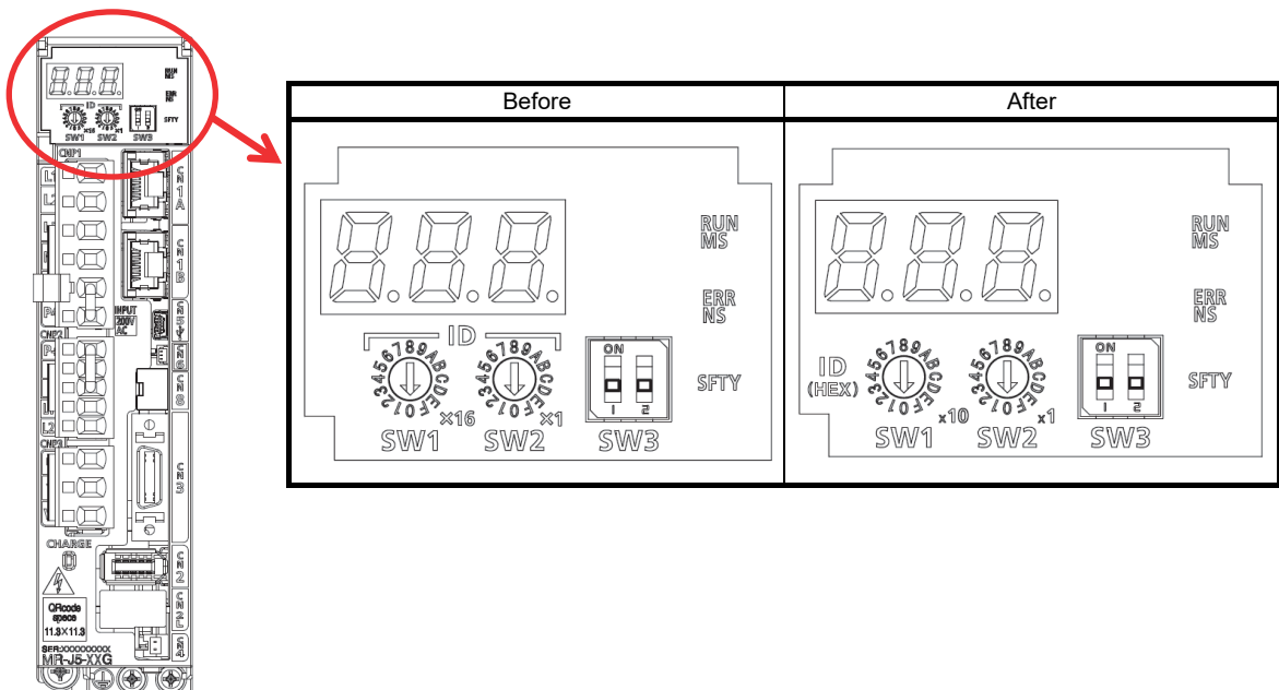
Figure 1. Rotary switch indication change (for MR-J5-10G-N1)
