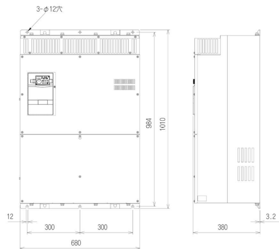
■FR-A740-220K, 250K, 280K
