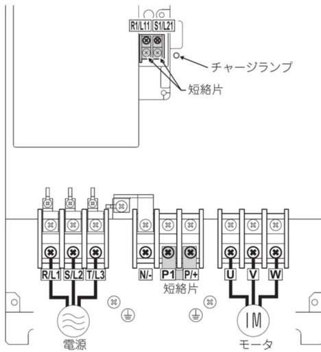
■FR-A740-30K, 37K, 45K
