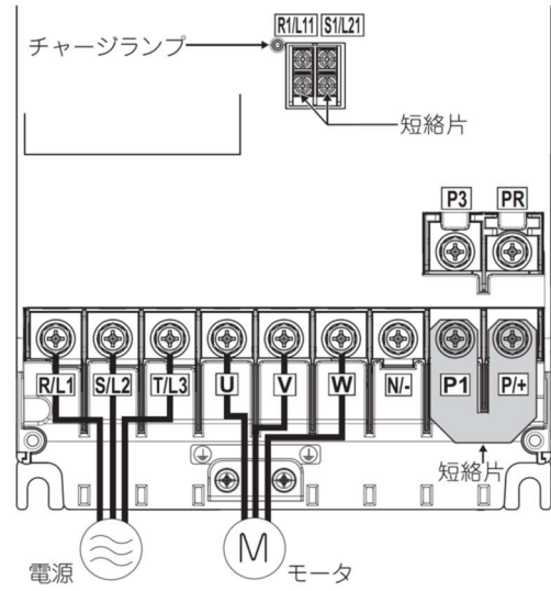
■FR-A840-18. 5K, 22K
