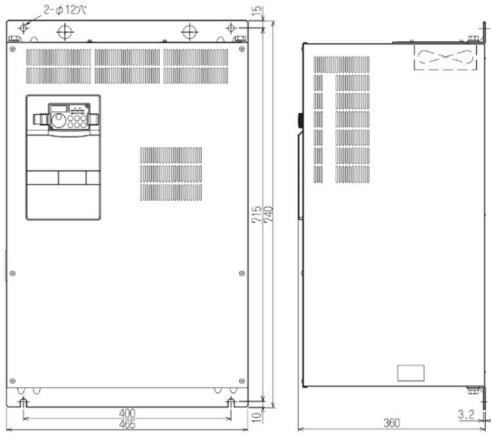
■FR-A740-110K, 132K
