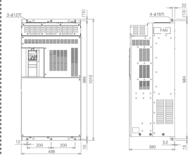
■FR-A840-160K, 185K
