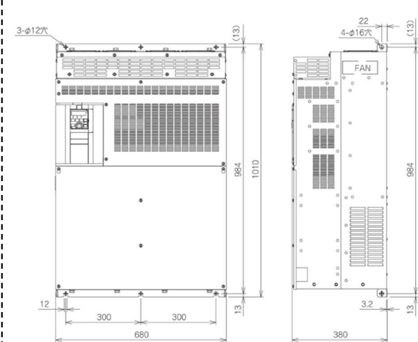
■FR-A840-220K, 250K, 280K
