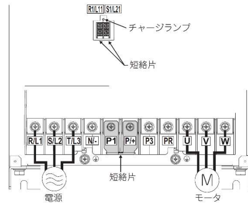
■FR-A840-37K, 45K, 55K
