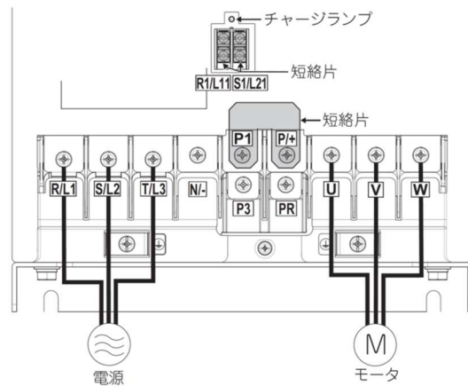
■FR-A840-30K
