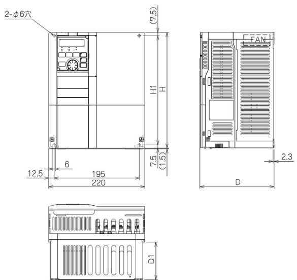
■FR-A820-5.5K, 7.5K
