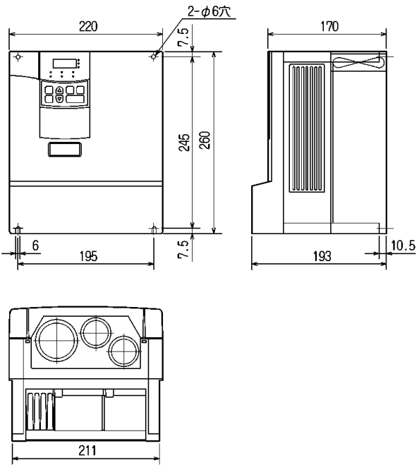
■FR-V520-3.7K, 5.5K
