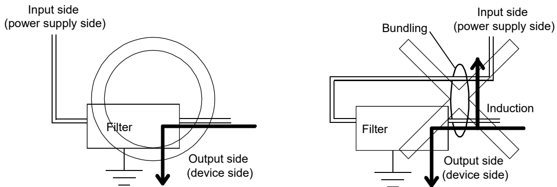
Fig. 2 Precautions on noise filter
