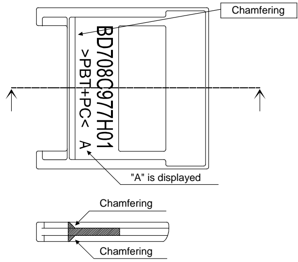
Figure 3 The dummy CompactFlash card ("A" is displayed)
