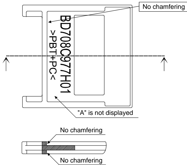
Figure 2 The dummy CompactFlash card ("A" is not displayed)
