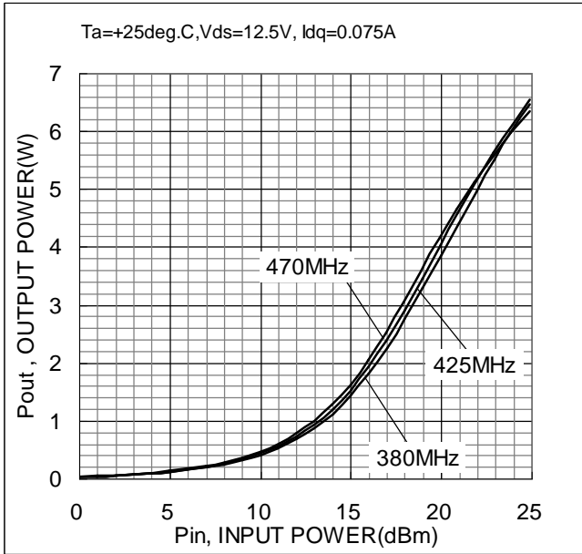
INPUT POWER (Vds=12.5V)
