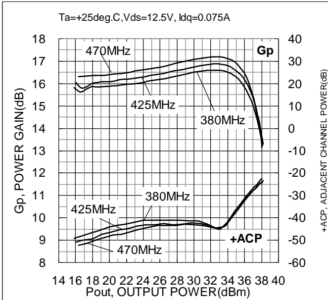
POWER GAIN and +/- ADJACENT CHANNEL POWER (Vds=12.5V)
