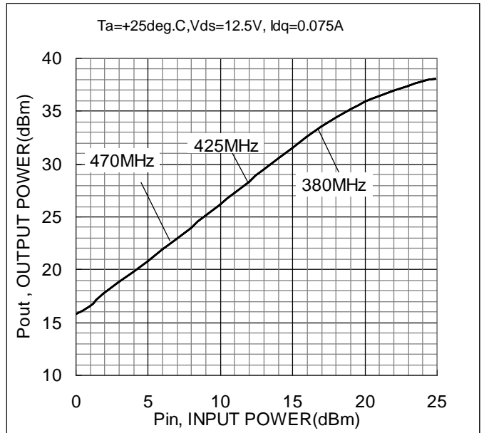
INPUT POWER (Vds=12.5V)
