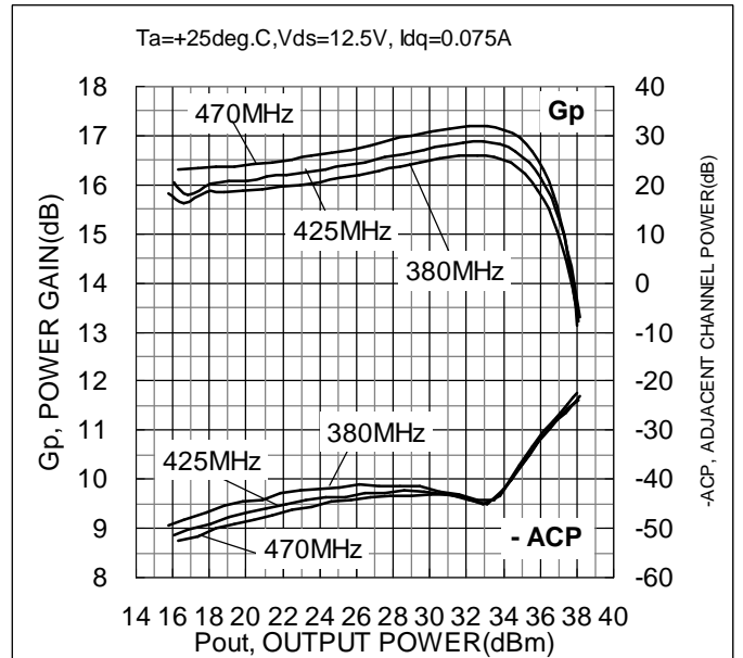
POWER GAIN and +/- ADJACENT CHANNEL POWER (Vds=12.5V)
