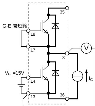
G-E 間短絡 GUP-EUP, GUN-EUN, GVP-EVP, GVN-EVN, GB-EB
