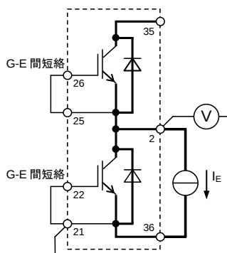
G-E 間短絡 GUP-EUP, GUN-EUN, GWP-EWP, GWN-EWN, GB-EB
