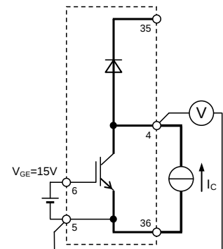
G-E 間短絡 GUP-EUP, GUN-EUN, GVP-EVP, GVN-EVN, GWP-EWP, GWN-EWN
