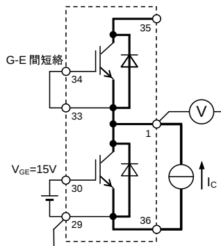
G-E 間短絡 GVP-EVP, GVN-EVN, GWP-EWP, GWN-EWN, GB-EB
