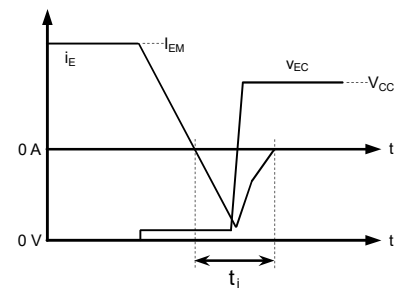
FWD/DIODE 逆回復損失
