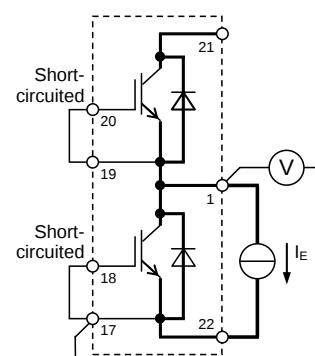
G-E 間短絡 GVP-EVP, GVN-EVP, GWP-EWN, GWN-EWN UP / UN FWD
