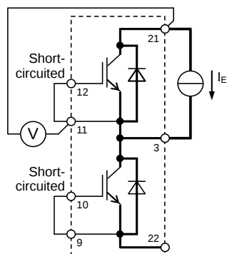
G-E 間短絡 GUP-EUP, GUN-EUN, GVP-EVP, GVN-EVN, WP / WN IGBT
