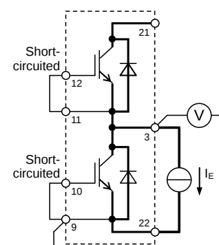
G-E 間短絡 GUP-EUP, GUN-EUN, GVP-EVP, GVN-EVN WP / WN FWD
