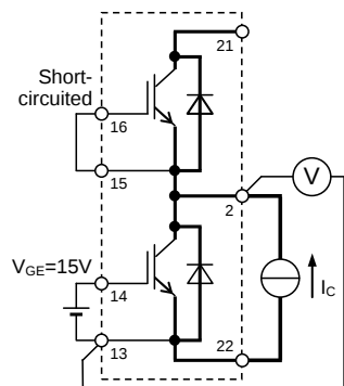
G-E 間短絡 GUP-EUP, GUN-EUN, GWP-EWP, GWN-EWN VP / VN IGBT
