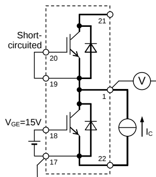
G-E 間短絡 GVP-EVP, GVN-EVP, GWP-EWN, GWN-EWN UP / UN IGBT
