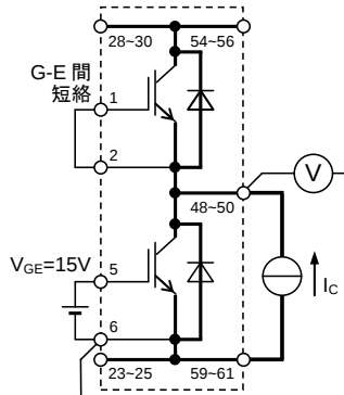
G-E 間短絡 GVP-EVP, GVN-EsVP, GWP-EWN, GWN-EsWN UP / UN IGBT
