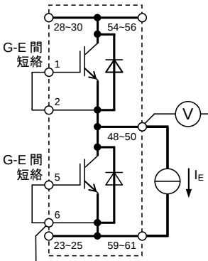
G-E 間短絡 GVP-EVP, GVN-EVP, GWP-EWN, GWN-EWN UP / UN FWD
