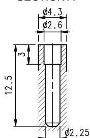
SECTION A
