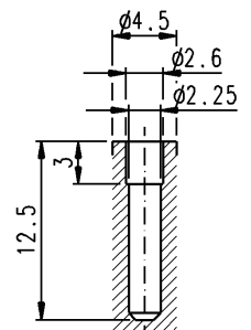
SECTION A
