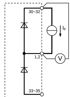
Brake IGBT/Diode
