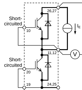
G-E 間短絡 GUP-U, GUN-E, GWP-W, GWN-E VP / VN IGBT
