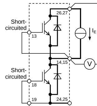
G-E 間短絡 GUP-U GUN-E, GVP-V, GVN-E WP / WN IGBT
