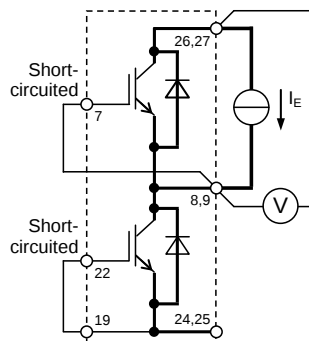
G-E 間短絡 GVP-V GVN-E, GWP-W, GWN-E UP / UN IGBT
