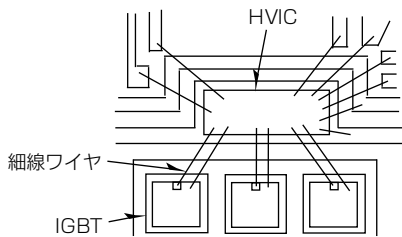
(b) DIPIPM+
